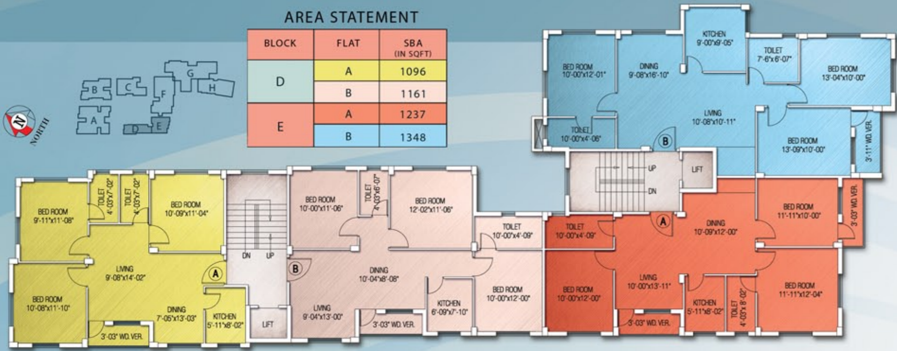
Typical Floor Plan - Block D & Block E
